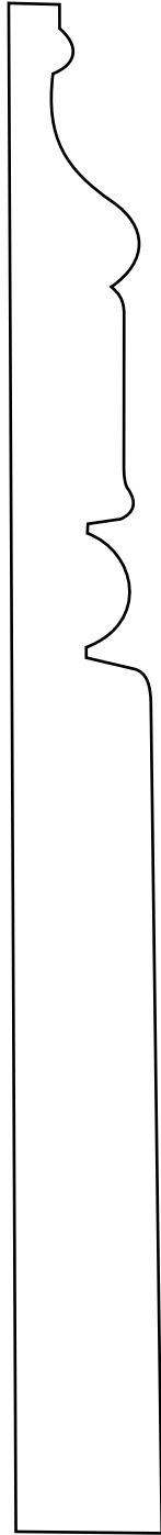
22232-eb-smooth 11/16 X 7-1/4 base
