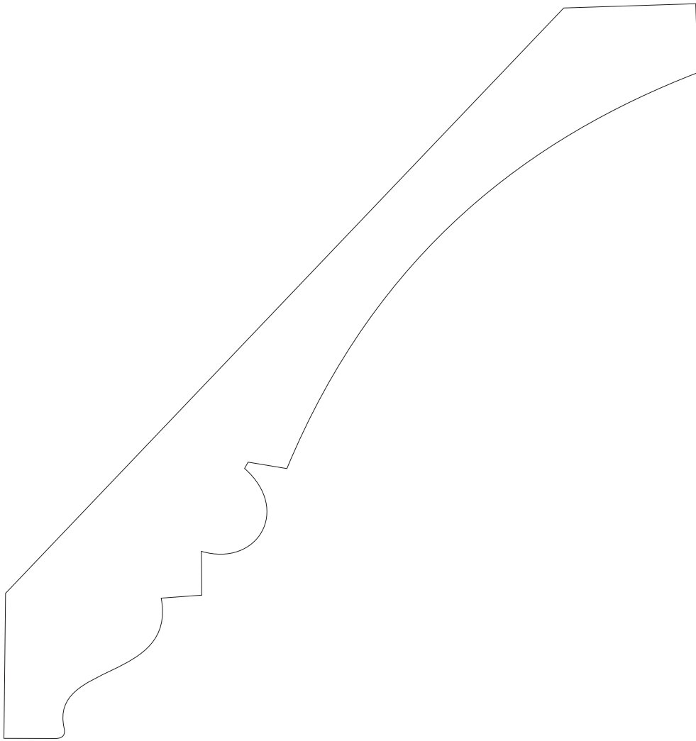
HM738-S 1-1/16 x 7-3/8 crown Copyright Flex Trim, Inc. 2005
