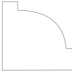
JMCA138-S 1-3/8 x 1-3/8 corner mold Copyright Flex Trim, Inc. 2005
