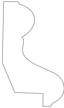
JMOLRPM-S 1-1/16 x 1-3/4 panel mold Copyright Flex Trim, Inc. 2005
