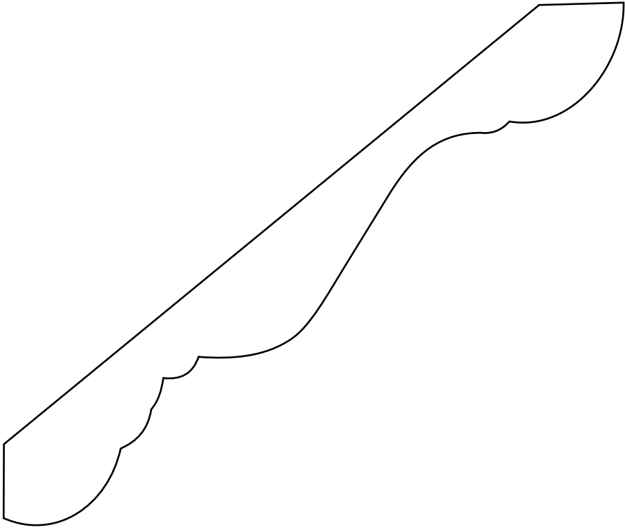
kcldf46-s 3/4 x 6 crown
