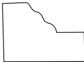
KCR619 ~ smooth 1 x 1-7/16 BRICK MOLD Copyright Flex Trim, Inc. 2005
