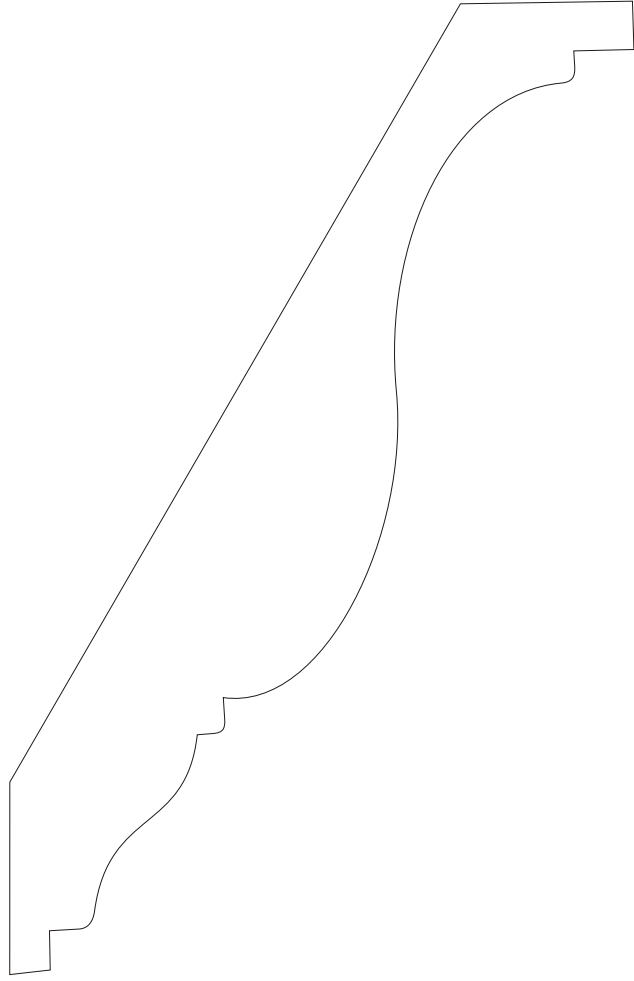
MMO11-S 1-1/16 x 5-7/8 crown Copyright Flex Trim, Inc. 2005
