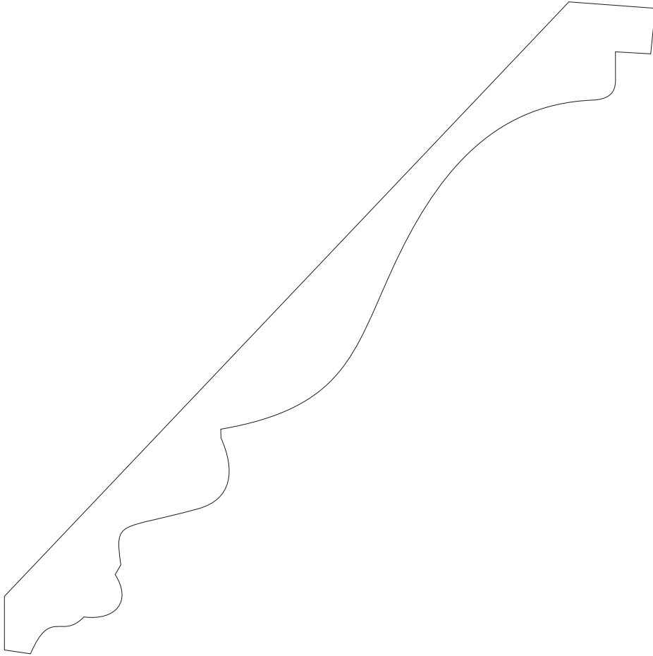
MM270M-S 11/16 x 6-3/4 crown Copyright Flex Trim, Inc. 2006
