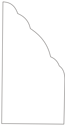
MVGLP911-S 1-1/4 x 2-1/4 lintel mold Copyright Flex Trim, Inc. 2005
