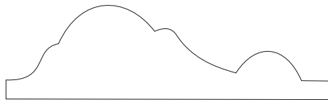
SS85-S 3/4 x 2-1/2 chair rail Copyright Flex Trim, Inc. 2005
