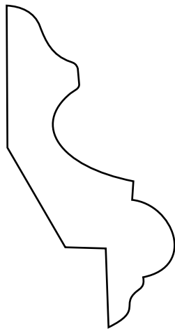
WBH1604 ~ smooth 3/4 x 2-1/2 PANEL MOLD
